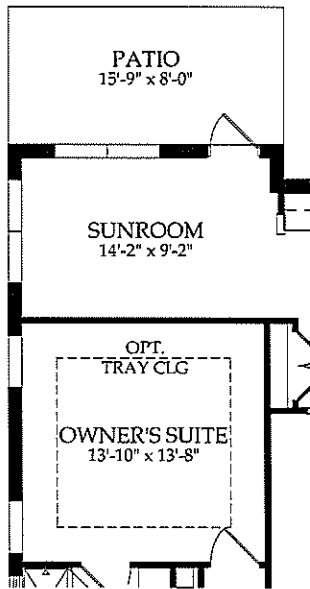
Sunroom Option
