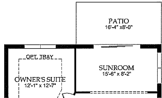
Sunroom Option
