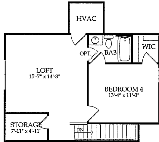
Loft with Bedroom and Bath
