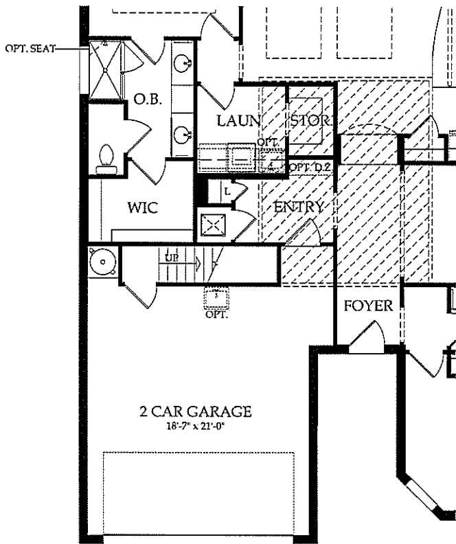
Attic Storage Option w/4' Garage Extension
