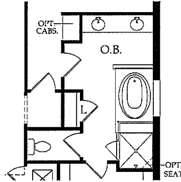
Tub Upgrade @ Owner's Bath
