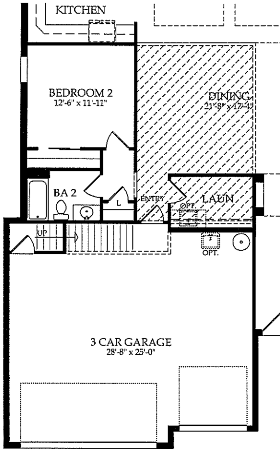
Attic Storage Option w/4' Garage Extension
