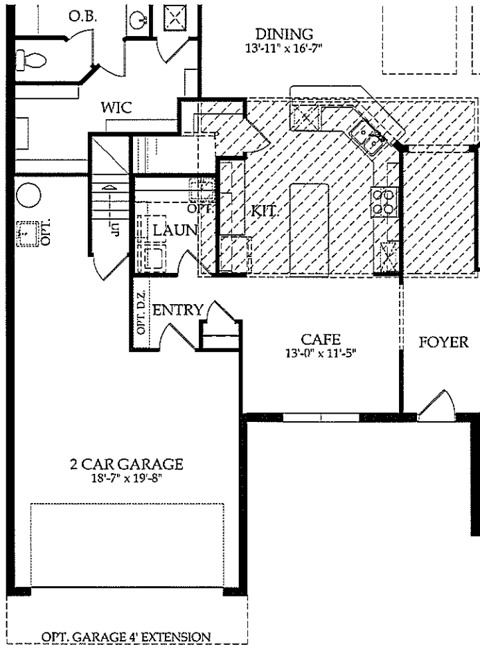
First Floor w/ Attic Storage
