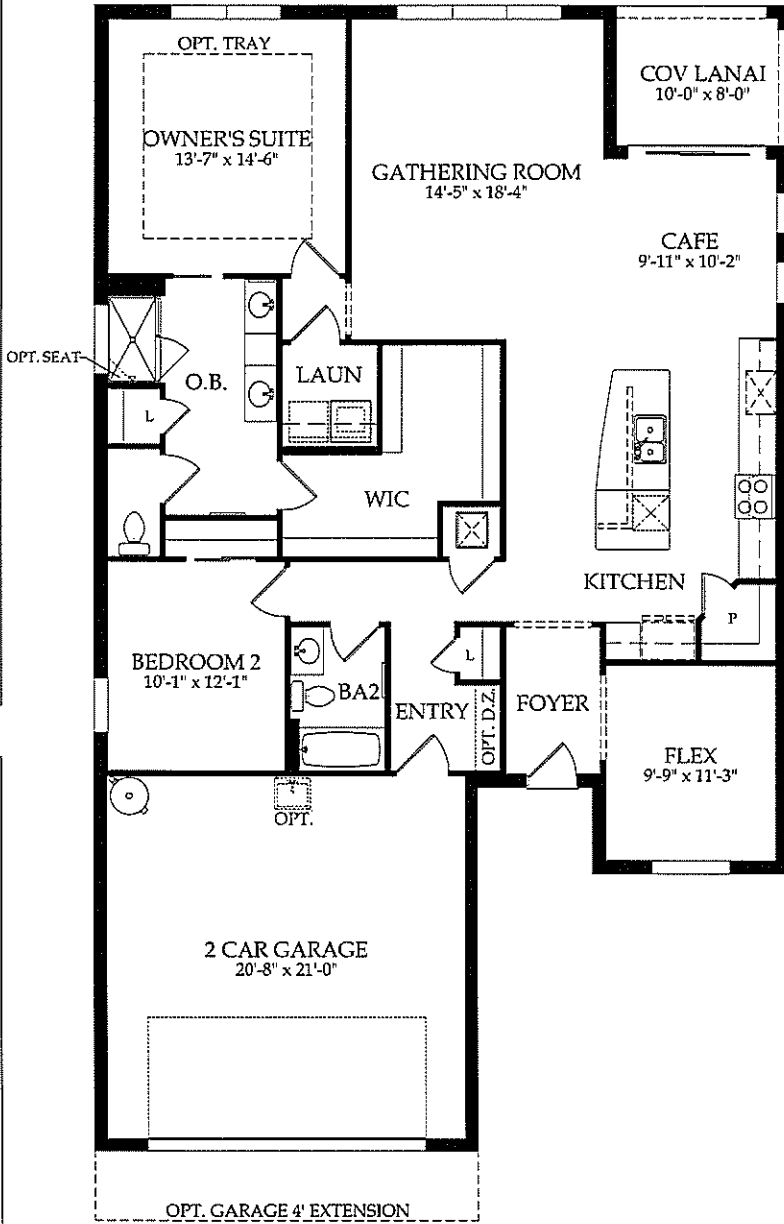
First Floor Elevation FM1A
