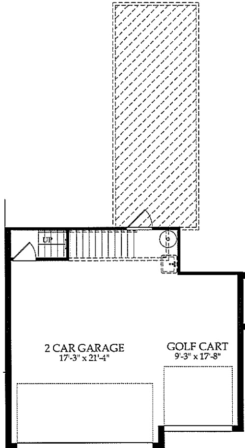
Attic Storage Opt. w/ 4' Garage Extension
