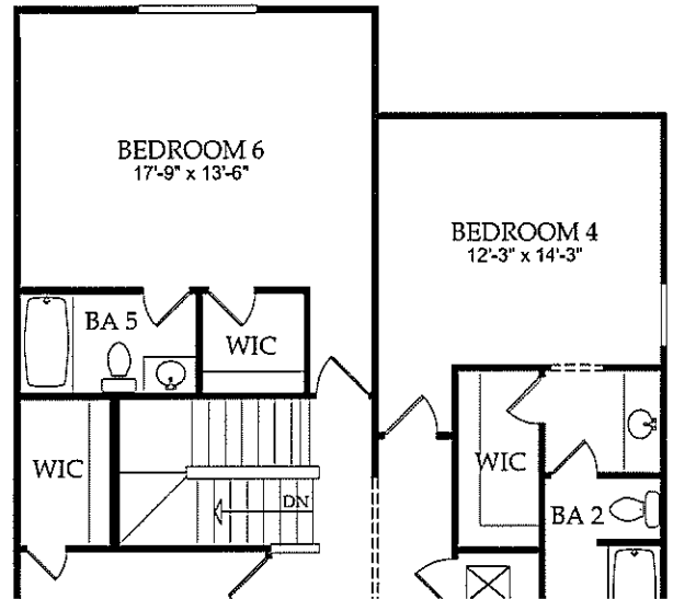
Bedroom 6 & Bath 5 Option
