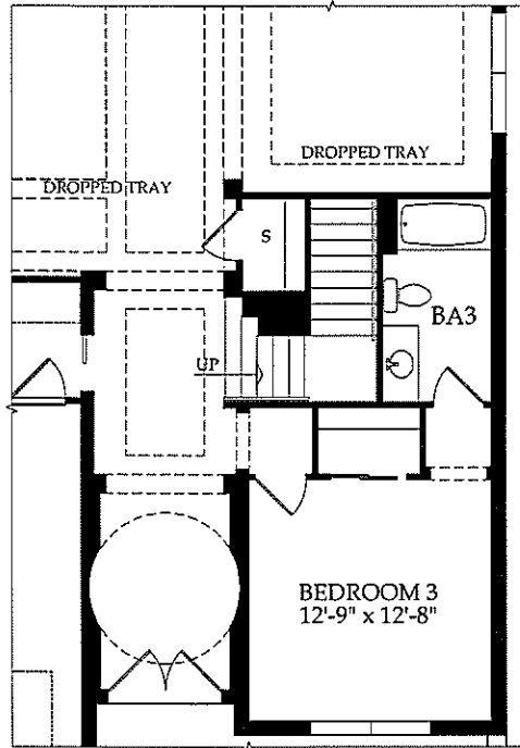
First Floor Plan w/ Opt Loft
